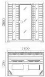
06-K6 Size:1800×1200×2000mm
