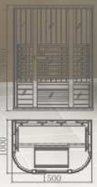
04-K71 Size:1500×1000×1980mm
