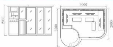
O6-K8 Size:3000×2500×2000mm
