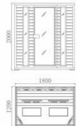
06-K6 Size:1800x1200x2000mm
